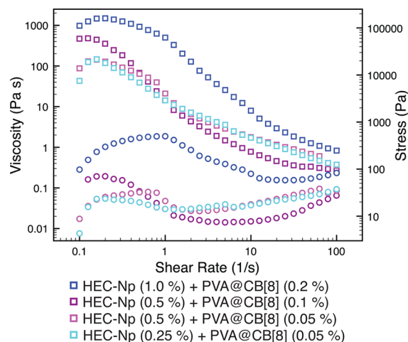
Figure 5. Steady-shear rheological measurements of the hydrogels demonstrating the response of the supramolecular hydrogels to constant-shear-induced deformation at 20 °C. The symbols and legend denotations are as above.
