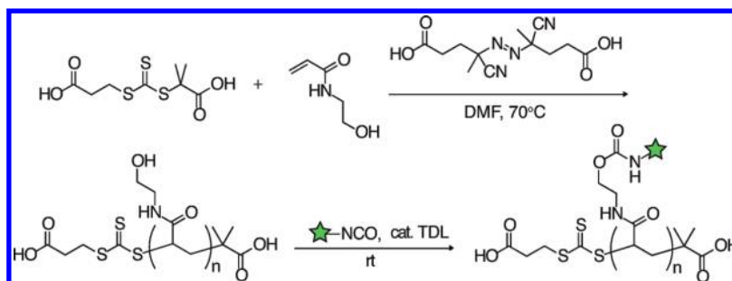
Scheme 5. Reaction Scheme for the Preparation of Side-Chain Functional Polymers by Isocyanate Conjugation to a Hydroxyl-Pendant Polymer, Poly( N -hydroxyethylacrylamide) (PHEAm), Prepared by Reversible Addition–Fragmentation Chain Transfer (RAFT) Polymerization
