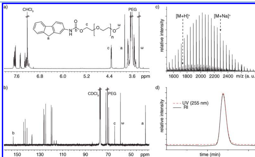
Figure 1. Characterization of FO-PEG-OMe (2000 g mol -1 ) by (a) 1 H NMR, (b) 13 C NMR, (c) high-resolution ESI-MS, and (d) GPC. These methods confirm the high degree of end-group functionalization (>99%) as well as excellent purity of the material, most notably the absence of the potential oxidation byproduct fluorenone.
