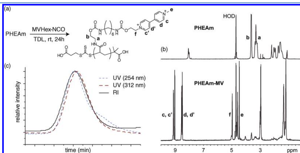
Figure 3. Characterization of PHEAm–MV, shown in (a) by 1 H NMR (b) and GPC (c). Comparison of the 1 H NMR spectra of the starting polymer PHEAm (top) and the MVHex conjugated polymer PHEAm–MV (bottom) confirms the degree of functionalization (70%). This is supported by the overlay of GPC traces from the refractive index (RI), UV at 254 nm resulting from the MVHex functionality, and the UV at 312 nm resulting from the trithiocarbonate end group on the polymer.
