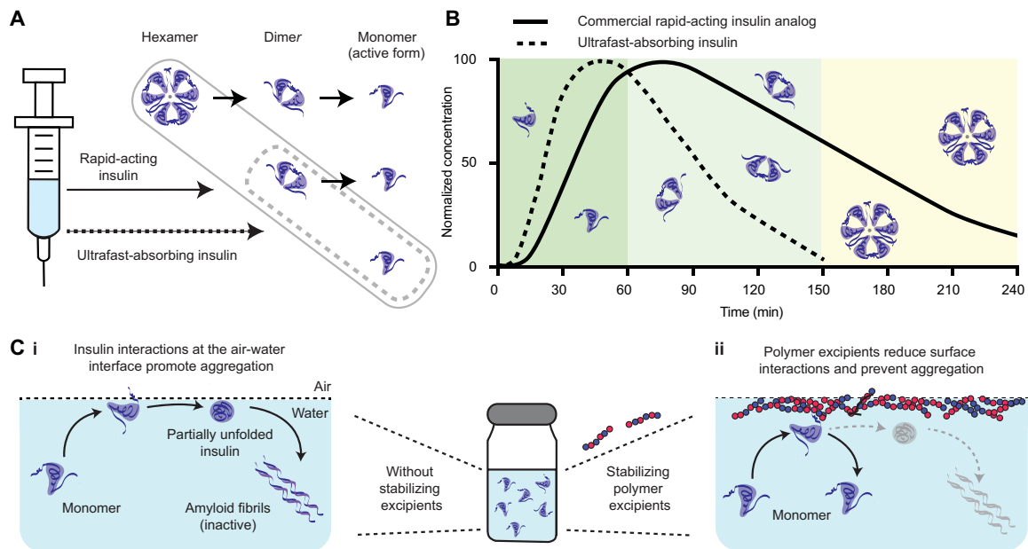
Fig. 1. Scheme of absorption kinetics of the various association states of insulin. (A) Commercial rapid-acting insulin (RAI) formulations contain a mixture of insulin hexamers, dimers, and monomers. Only the monomeric form of insulin is active; thus, the dissociation from the hexamer to the monomer is rate limiting for therapeutic action. An ultrafast insulin formulation would contain primarily insulin monomers and no insulin hexamers for rapid insulin absorption after subcutaneous administration. (B) A schematic illustrating the contribution of insulin hexamers, dimers, and monomers in commercial RAI formulations to the observed duration of insulin action when delivered subcutaneously in humans. Insulin monomers are absorbed in about 5 to 10 min, dimers are absorbed in 20 to 30 min, and hexamers can take 1 to 2 hours to be absorbed and result in prolonged insulin action accordingly. A primarily monomeric insulin formulation would reduce time to onset and result in shorter duration of insulin action for better management of blood glucose at mealtimes. (C) A hexamer-free ultrafast insulin formulation will face stability challenges due to the propensity for insulin monomers to aggregate into amyloid fibrils. (i) At the interface, exposure of hydrophobic domains during insulin-insulin interaction nucleates amyloid fiber formation. (ii) Stabilizing polymer excipients are drawn to the air-liquid interface, impeding the interfacial nucleation of insulin amyloidosis.
