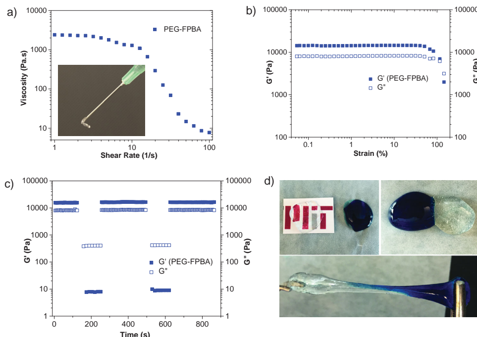
Figure 3. a) Viscosity and shear-thinning behavior of 10 w/v% PEG-FPBA gel. The inset shows that gel is injectable through a conventional syringe using a 21 G needle. b) Strain amplitude sweep. c) Step-strain measurements of 10 w/v% PEG-FPBA gel formed at pH 7. d) Demonstration of the self-healing properties of 10 w/v% PEG-FPBA gel, formed at pH 7, in fusing two hydrogel pieces. Gel was prepared in the presence of methylene blue for observation.
